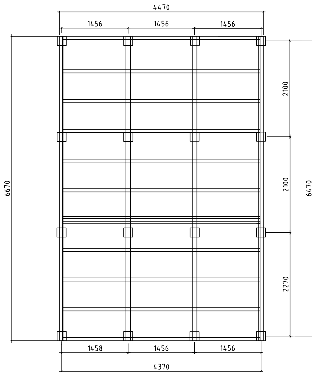
Scheme of base of camping house
