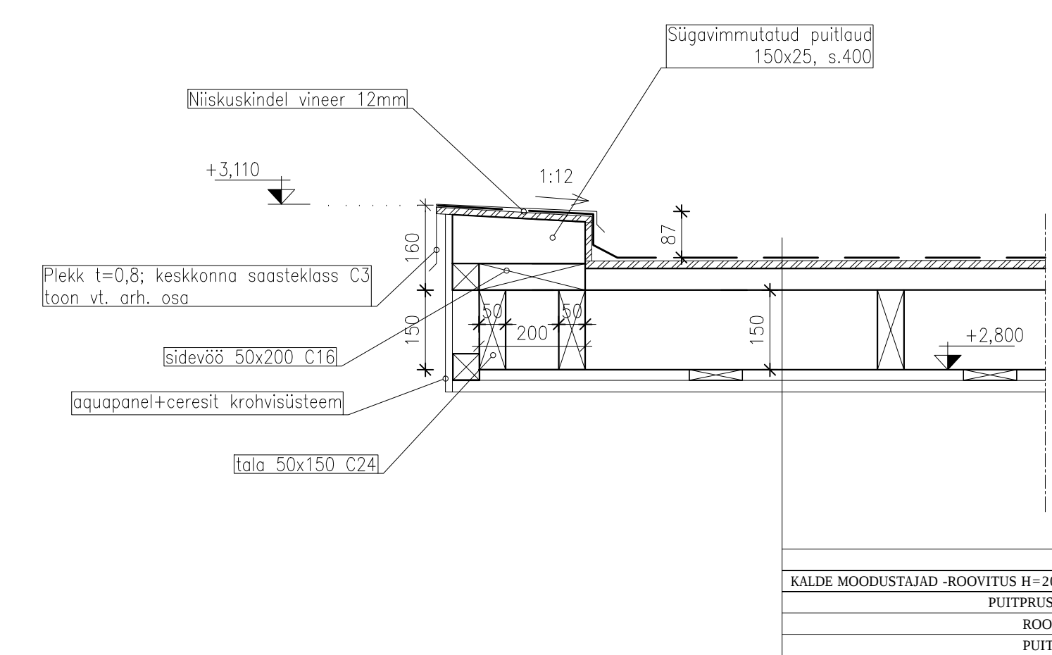
4vk-4vk M1:10
