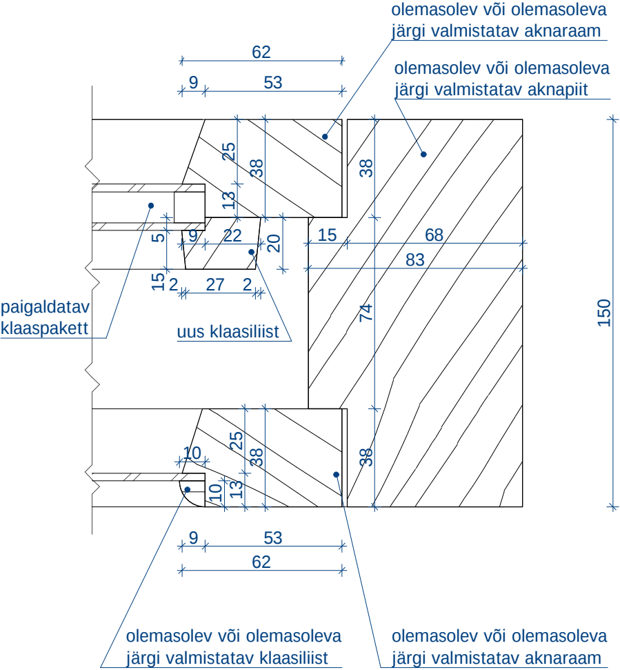
Detail "A11"
