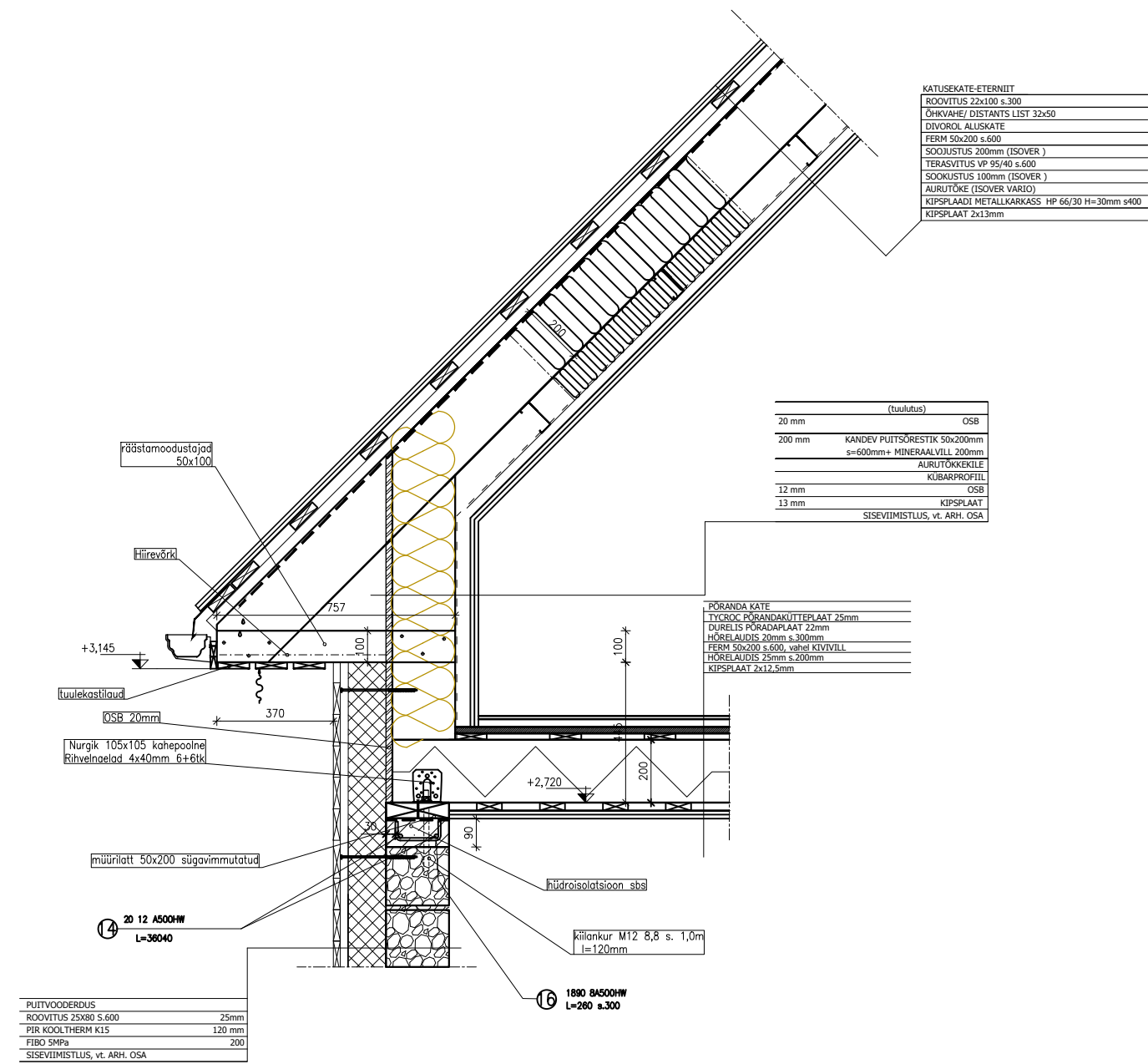
Detail "1" M1:10
