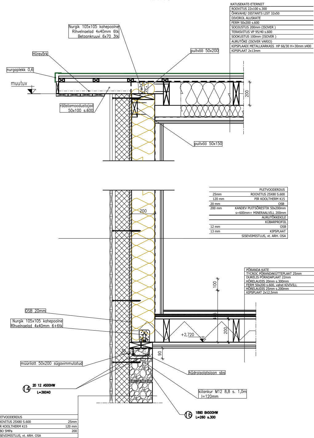
Detail "2" M1:10
