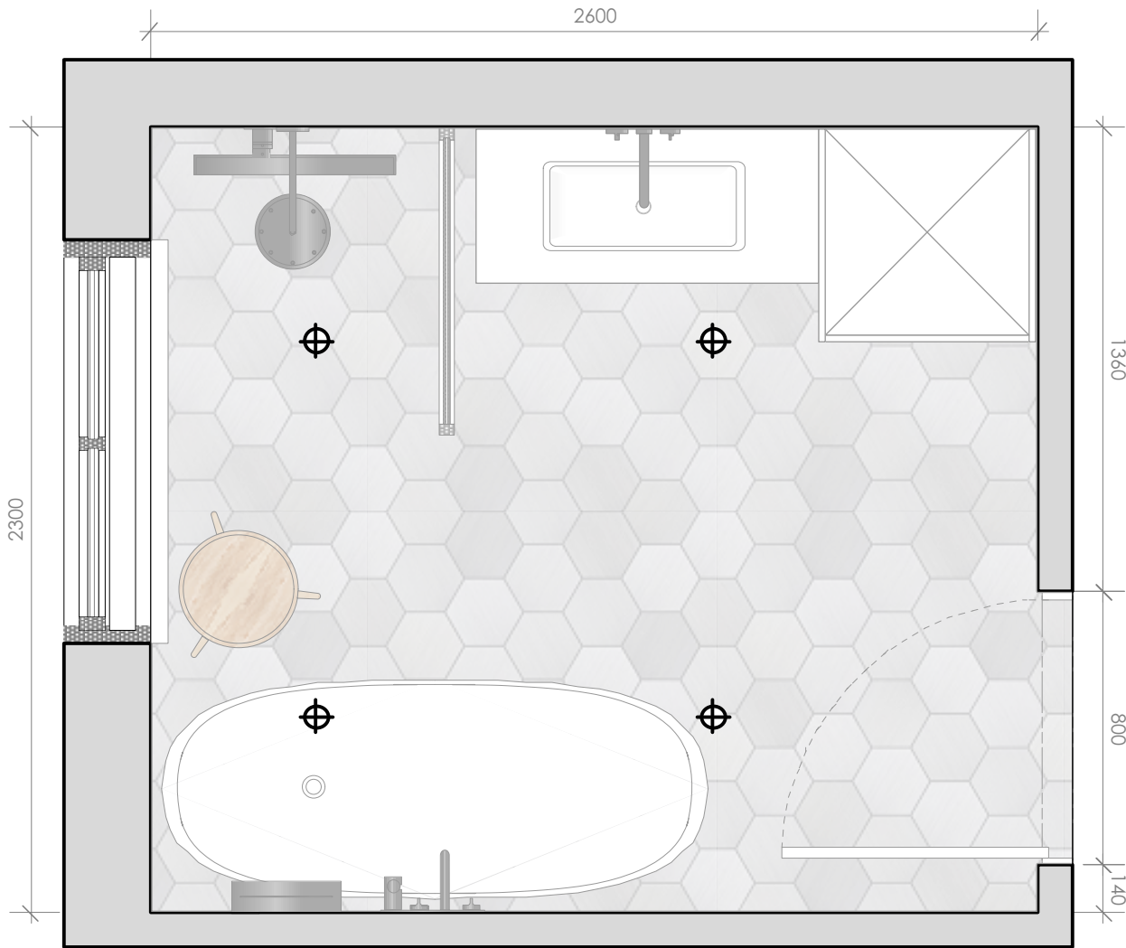
Floorplan - suggested ceiling lights
