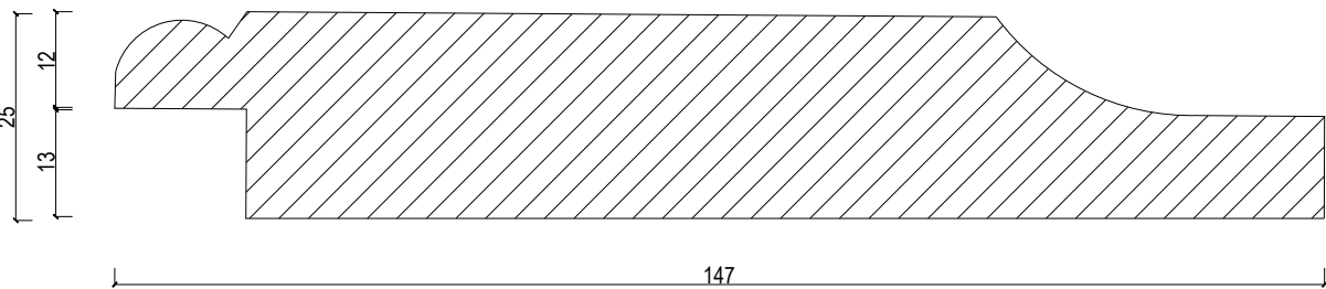
Stardilaud D-5 M 1:1 toon J460
