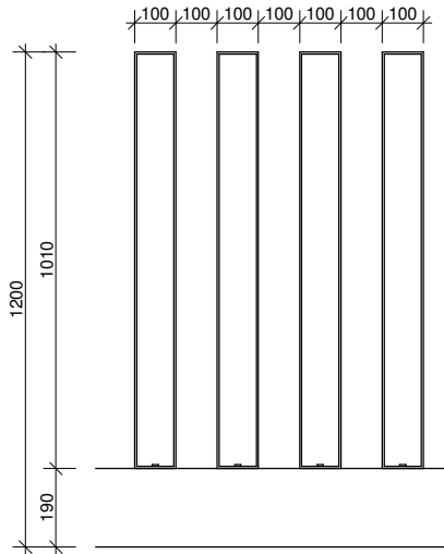
DETAIL 1:20
