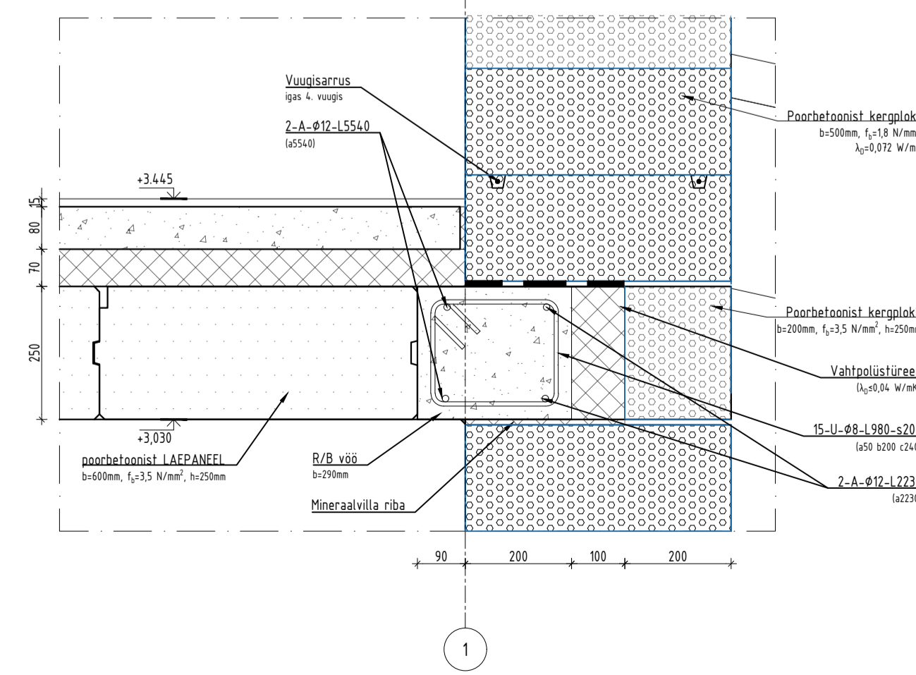
VLS-11 M1:10
