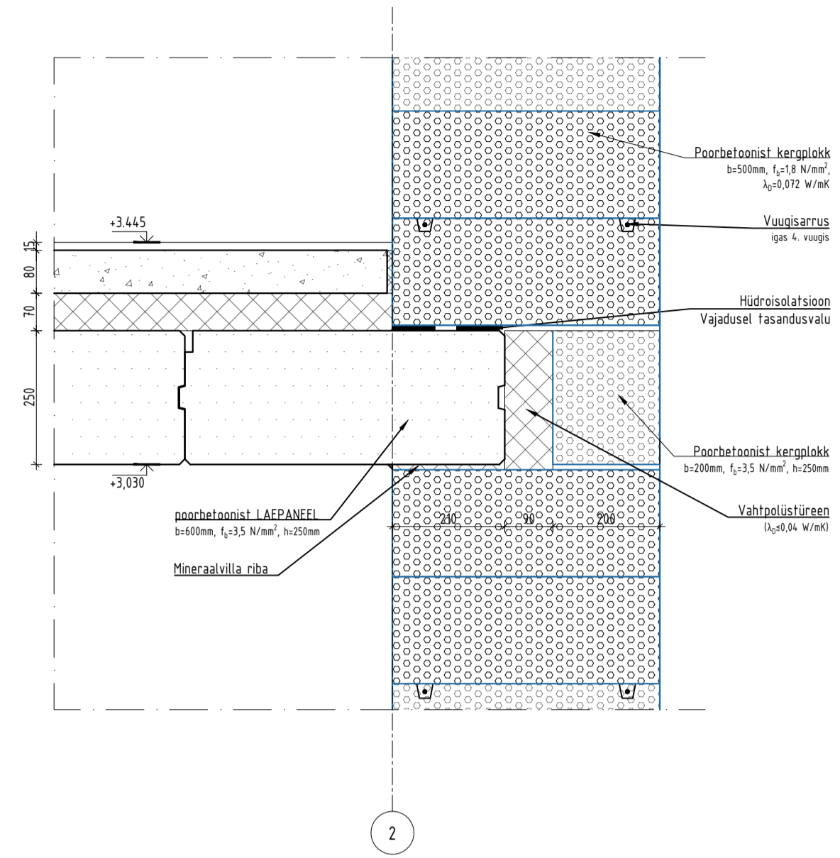
VLS-02 M1:10
