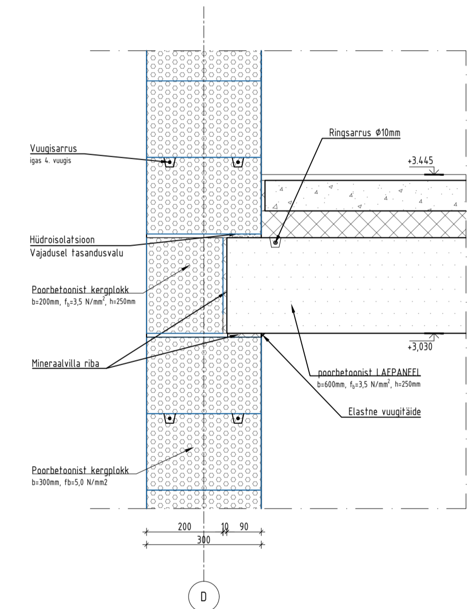
VLS-07 M1:10
