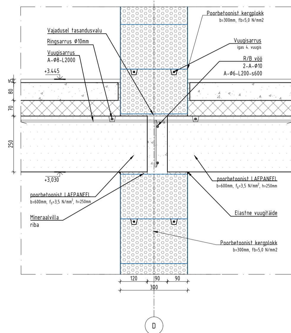
VLS-10 M1:10
