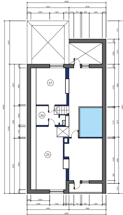
5 ATTIC FLOOR PLAN SCALE 1:200 M.
