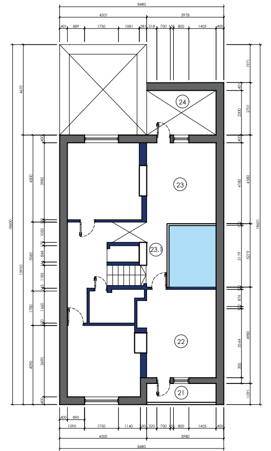
4 SECOND FLOOR PLAN SCALE 1:200 M.
