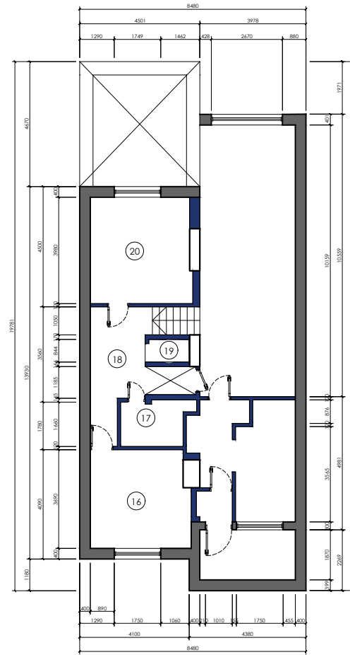
3 FIRST FLOOR PLAN SCALE 1:200 M.
