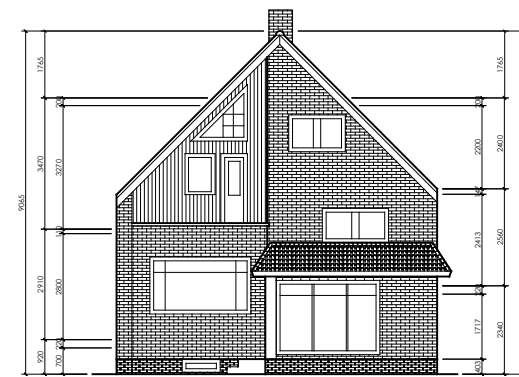
7 REAR ELEVATION SCALE 1:200 M.
