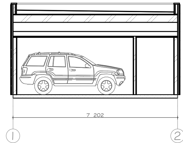
B Building Section 1:100
