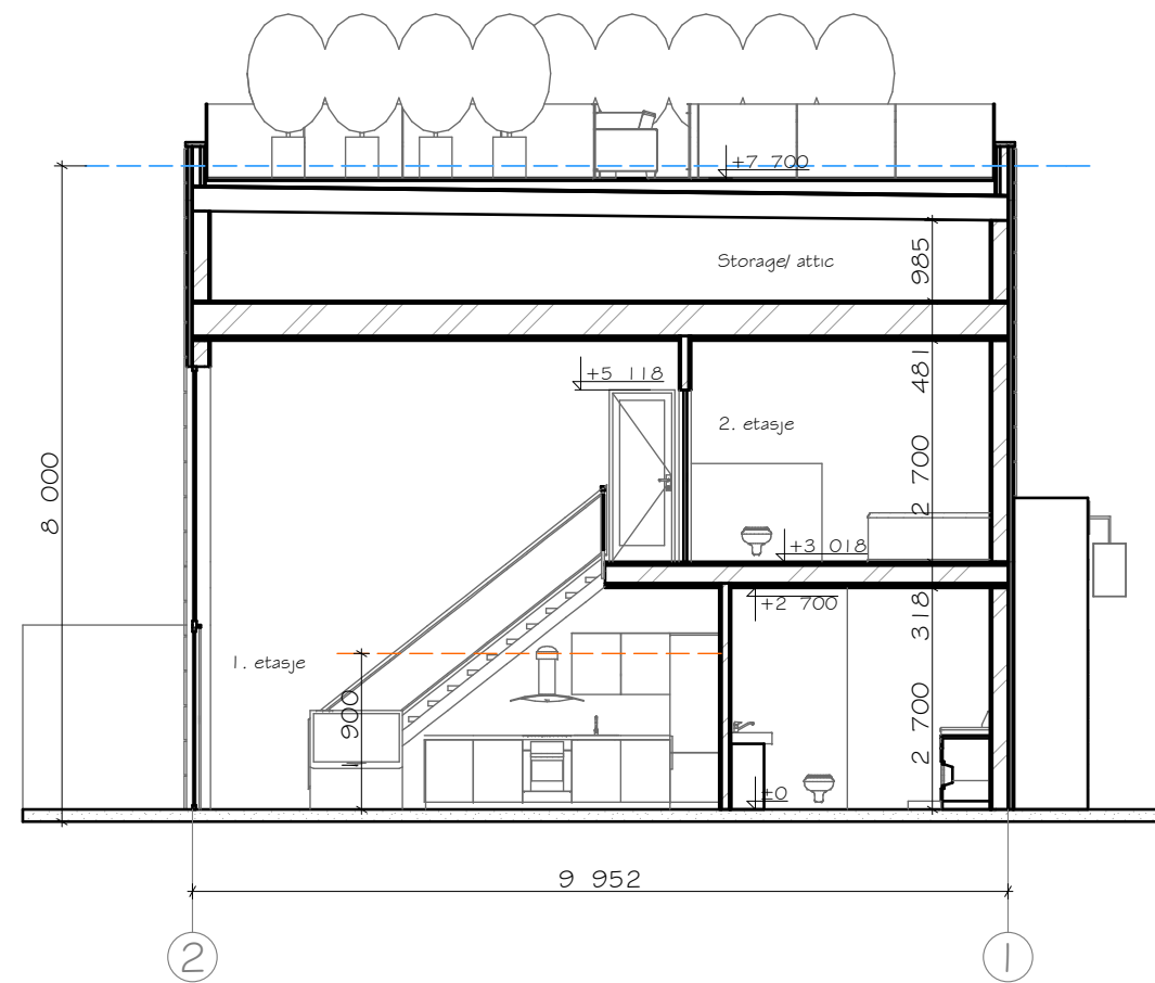
A Building Section 1:100
