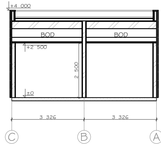
A Building Section 1:100
