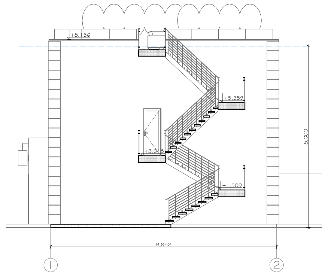
C Building Section 1:100
